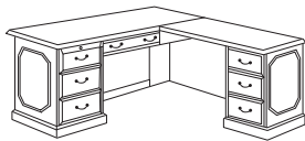
RIGHT EXECUTIVE L DESK 7350-28 (R) W66 D72 H30
